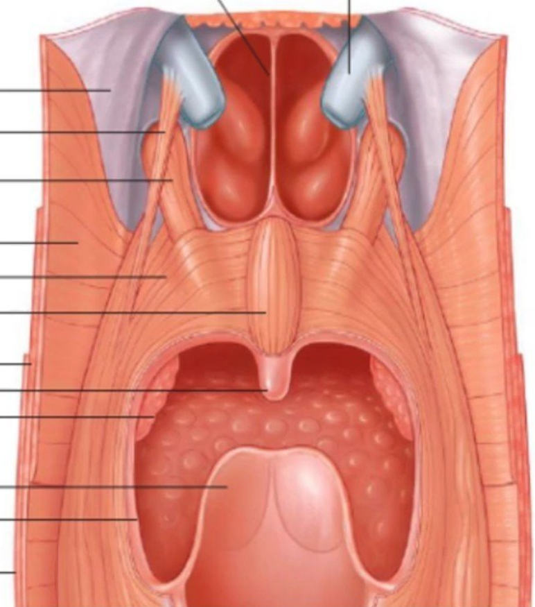
Muscles of the soft palate (posterior view)
